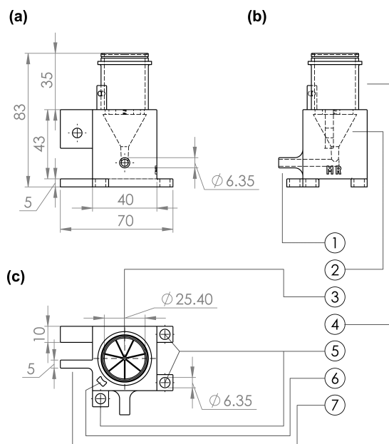
Figure 1. Dimensioned drawings of PRIZE: (a) rear view; (b) side view; (c) top view. All dimensions are in millimeters. The generator body consists of seven components: (1) inlet, (2) internal cone, (3) radial grid with openings, (4) elutriator tube, (5) mounting holes, (6) LED mount and (7) rotameter (or other flow meter) mount.
