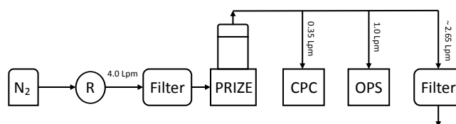
Figure 3. Schematic of the experimental setup used in this study. A filtered dry nitrogen flow was controlled by a rotameter (R) upstream of PRIZE. Downstream, the flow was split into three parts to a CPC, an OPS and excess flow discarded through a filter.
