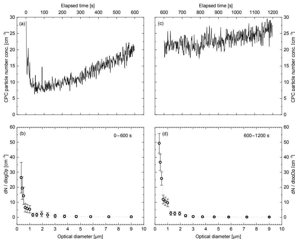
Figure 6. Arizona Test Dust measurements: (a) particle number concentration for the first 600 s; (b) corresponding particle size distribution; (c) particle number concentration for the second 600 s; (d) corresponding particle size distribution.
