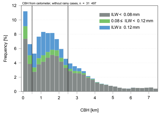
Figure 3. Cloud base heights (CBHs) from the ceilometer in Payerne with the corresponding integrated liquid water (ILW) from HATPRO (Humidity And Temperature PROfiler) in the years 2014 and 2015. The three different CBH classes (low, medium, and high) are indicated by the vertical black lines.
