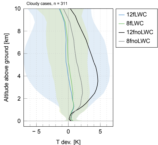
Figure 9. Mean bias with standard deviation (shaded area) when a simple cloud model is considered in the retrieval using all 12 frequency channels (12f, blue) and only 8 channels (8f, green) in the years 2014 and 2015. The mean biases for the same retrievals without considering clouds are given by the black (12 channels) and grey (8 channels) lines.
