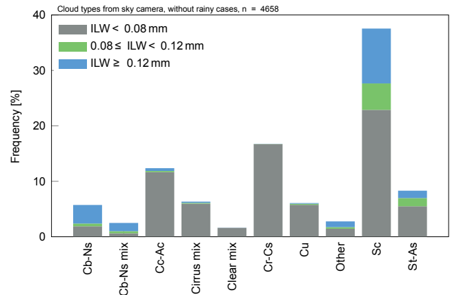
Figure 5. Cloud types detected by the sky camera in Payerne (2014–2015) and the corresponding ILW values from HATPRO. The different types are cumulonimbus–nimbostratus (Cb-Ns), mix of cumulonimbus–nimbostratus and another type (Cb-Ns mix, containing Cb-Ns and Cu, Sc, or St-As), cirrocumulus–altocumulus (Cc-Ac), cirrus mix (containing Cc-Ac or Cr-Cs clouds mixed with Cb-Ns, Cr-Cs, Cu, Sc, or St-As), clear mix (mix of cloud-free and another type), cirrus–cirrostratus (Cr-Cs), cumulus (Cu), other (containing cases where Sc was detected together with Cu or St-As), stratocumulus (Sc), and stratus–altostratus (St-As).
