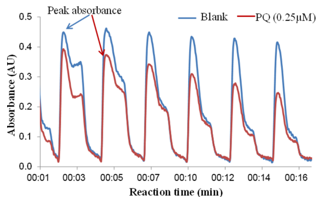
Figure 3. Peak absorbance for water blanks and PQ (0.25 \mu\text{M} ) after rinsing injection with water.
