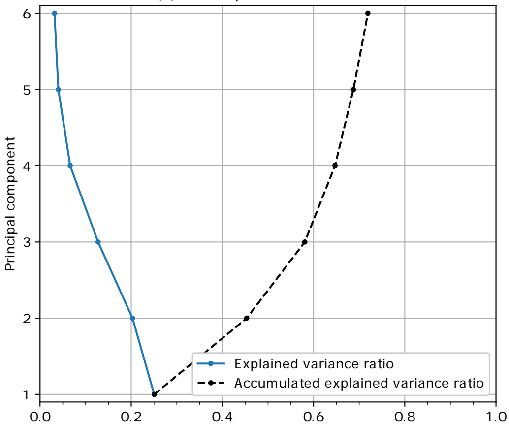
(b) M2: explained variance ratio
