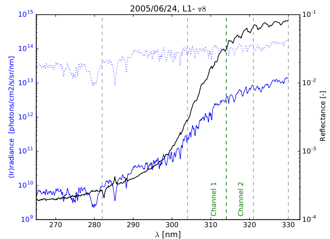
Figure 1. Example of SCIAMACHY spectra used for ozone profile retrieval: Earth radiance (solid blue line) and solar irradiance (dotted blue line) in photons \text{cm}^{-2}\text{ s}^{-1}\text{ sr}^{-1}\text{ nm}^{-1} , and reflectance (solid black line) (unit-less). The vertical dashed line in green separates the two channels and the vertical grey lines separate the clusters listed in Table 1.
