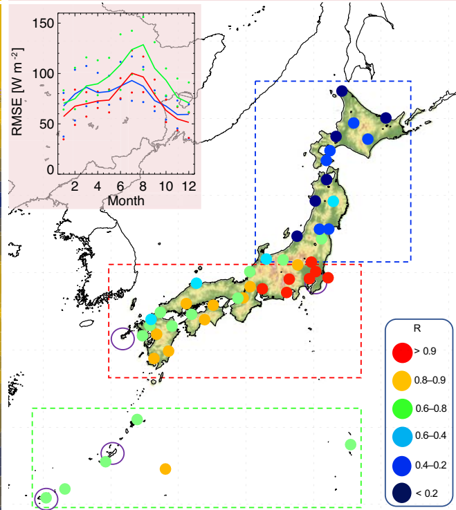
(b) Correlation between RMSE and cloud fraction in 2016
