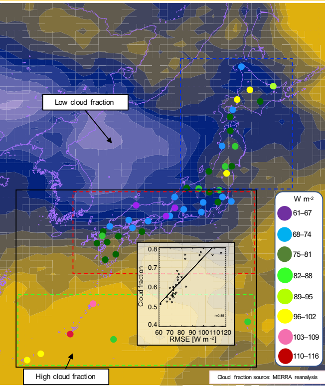
(a) Cloudiness vs. RMSE of JMA and H-8 in May 2016
