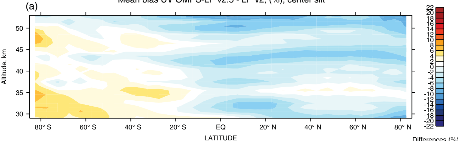
Mean bias UV OMPS-LP v2.5 - LP v2, (%), center slit
