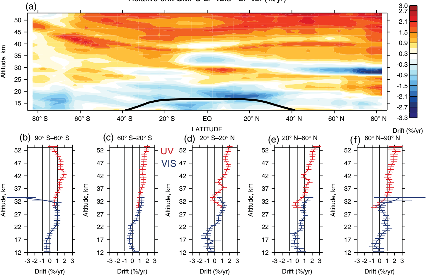
Relative drift OMPS-LP v2.5 - LP v2, (%/yr)
