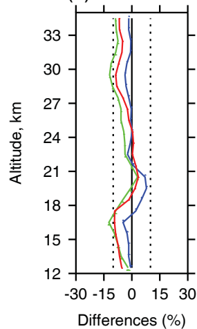
(f) 20° N–60° N
