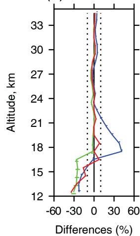
(e) 20° S–20° N
