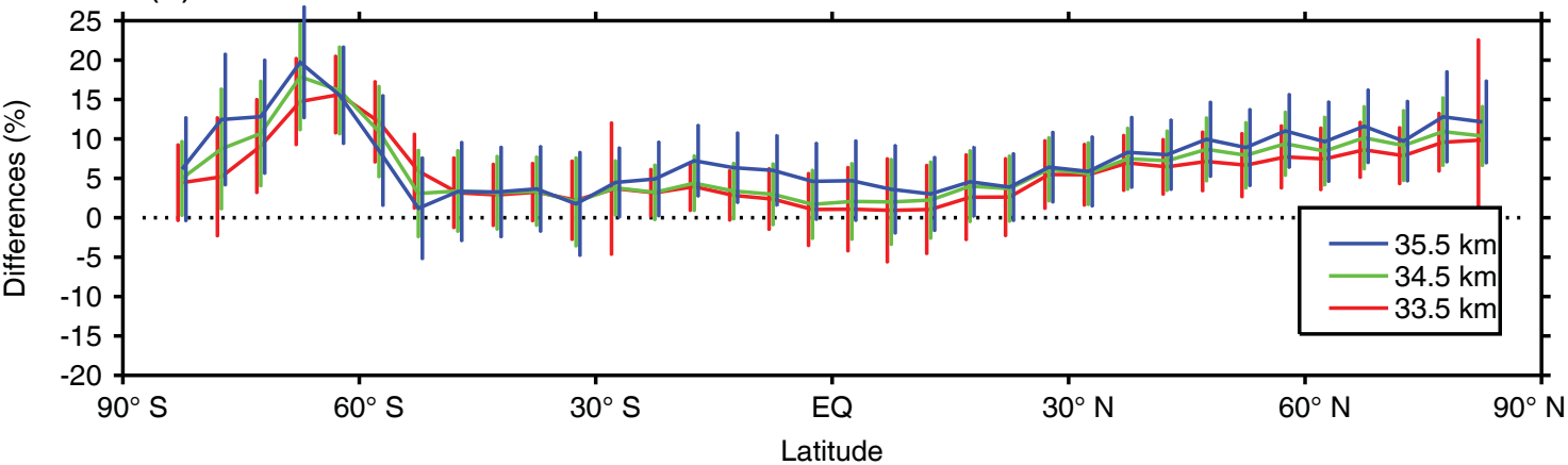
(b) Biases between UV and VIS ozone retrievals, LP v2.5
