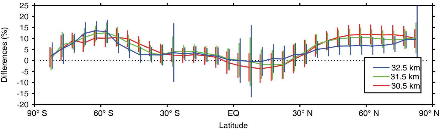
(a) Biases between UV and VIS ozone retrievals, LP v2.5
