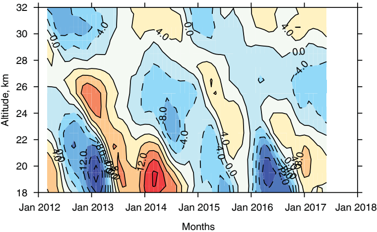
(a) OMPS-LP v2.5 ozone [%], 5° S–5° N
