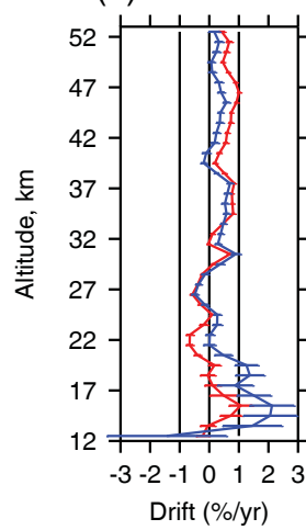
(e) 20° S–20° N
