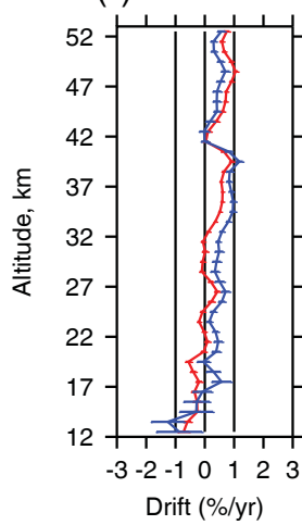
(f) 20° N–60° N
