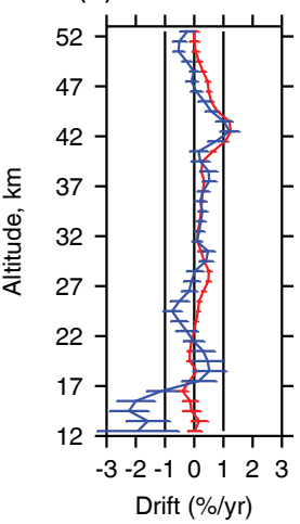
(c) 90° S–60° S
