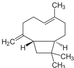
\beta -caryophyllene
