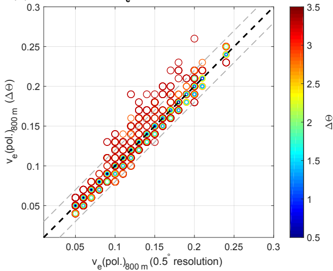
(b) Sensitivity of v_e (pol) to angular resolution
