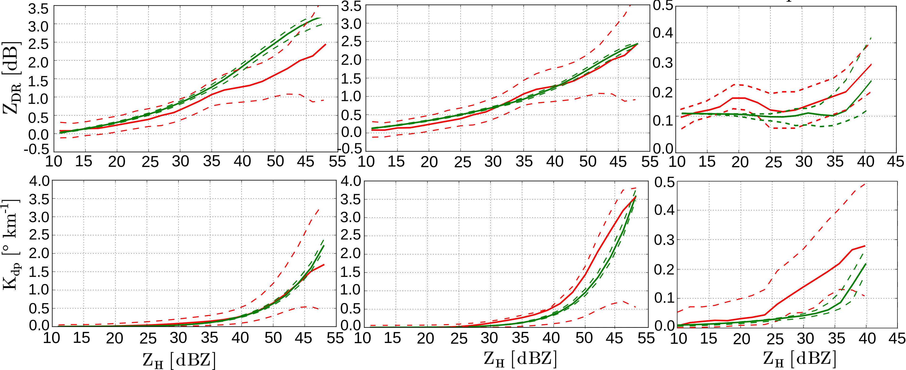
Liquid phase: \mu = 0.5
