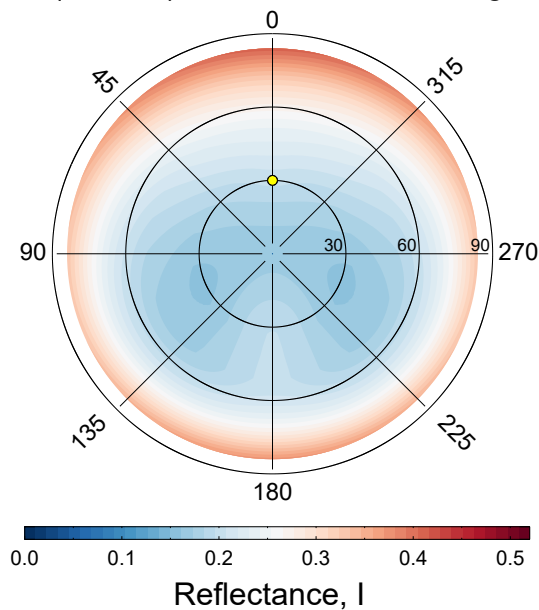
(a) BRDF (410 nm) for Maritime-ocean scene AOT (555 nm)=0.15, solar zenith angle=30°
