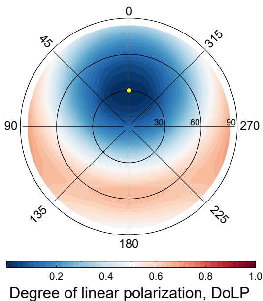
(c) BPDF (410 nm) for Maritime-ocean scene AOT (555 nm)=0.15, solar zenith angle=30°
