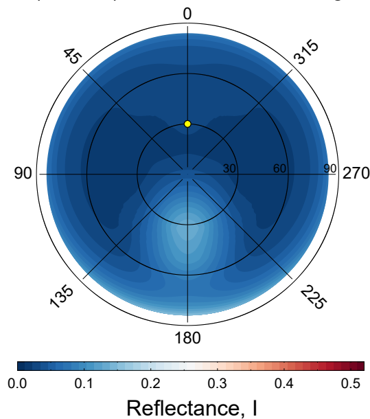
(b) BRDF (865 nm) for Maritime-ocean scene AOT (555 nm)=0.15, solar zenith angle=30°
