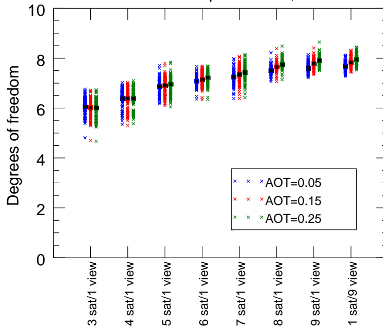
Reflectance + polarization, Land
