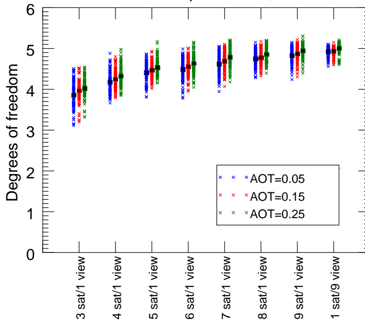
Reflectance + polarization, Ocean
