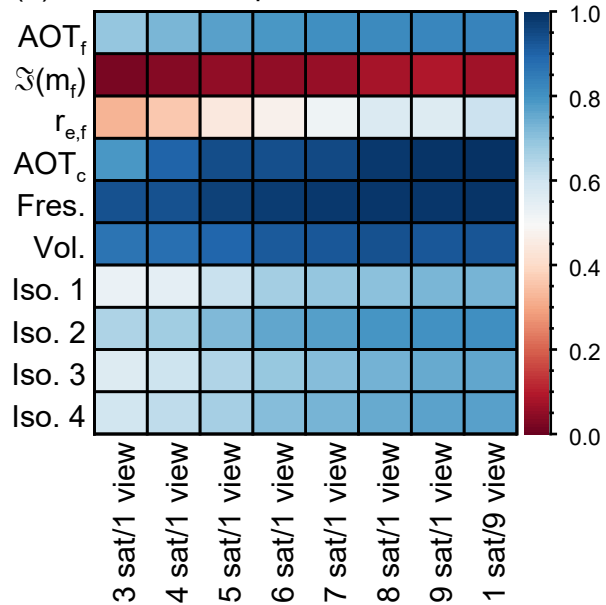
(b) Reflectance + polarization, Land AOT=0.1
