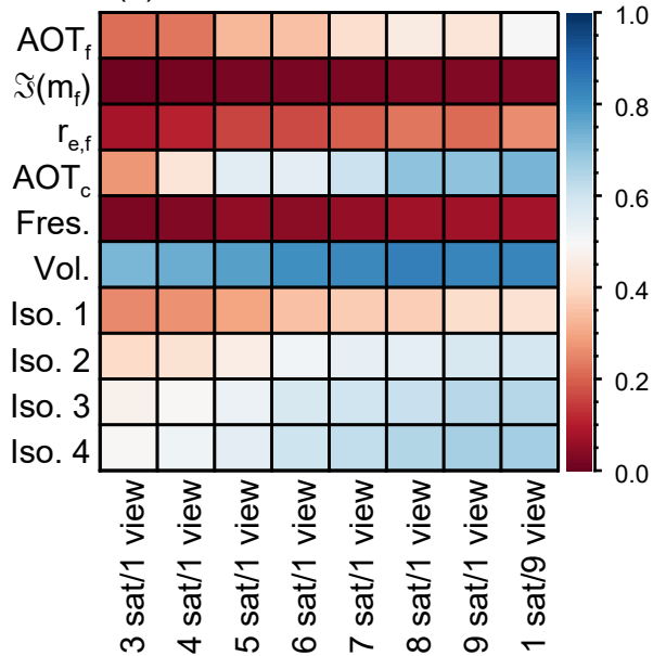
(a) Reflectance, Land AOT=0.15
