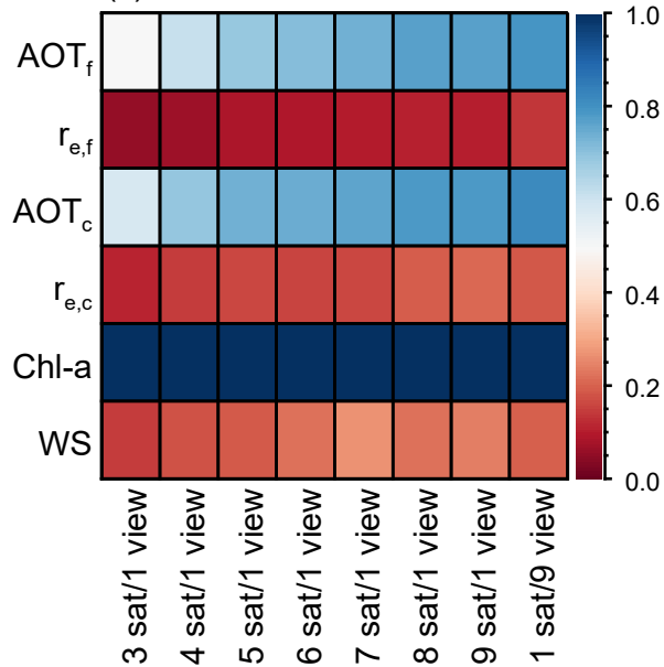
(c) Reflectance, Ocean AOT=0.15
