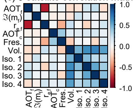
(c) 9 satellite correlation matrix
