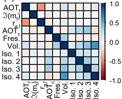
(a) 9 satellite correlation matrix
