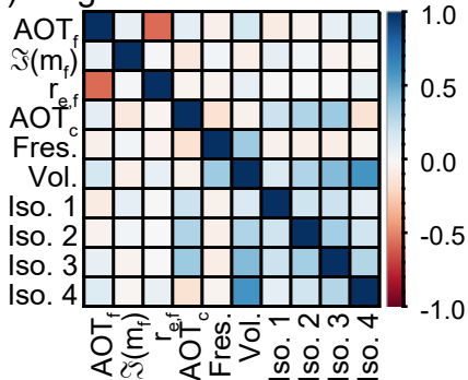
(b) Single satellite correlation matrix
