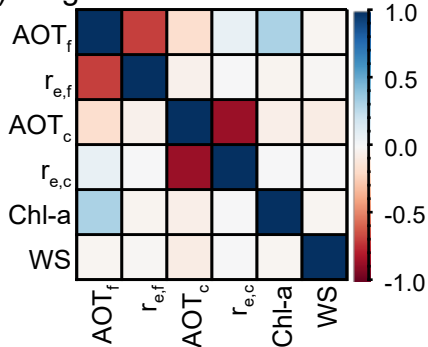
(f) Single satellite correlation matrix
