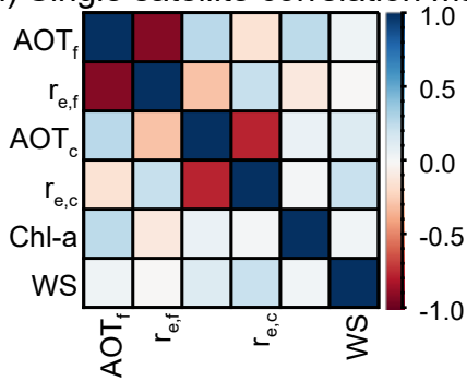
(h) Single satellite correlation matrix
