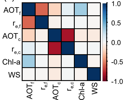
(e) 9 satellite correlation matrix
