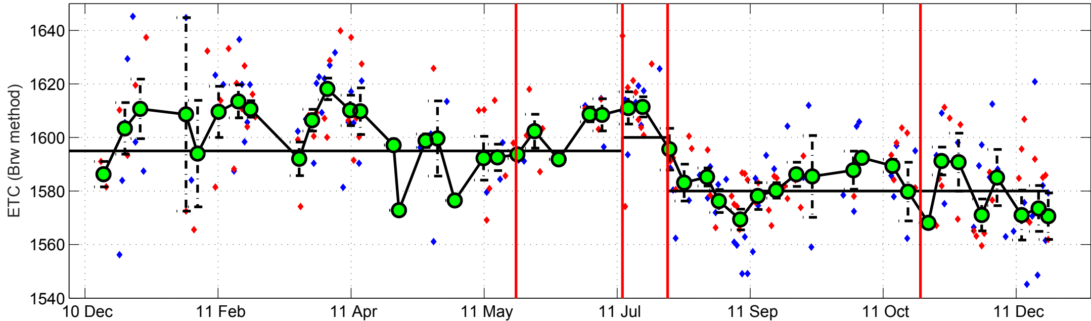
Langley plot (3 Jan 2011–25 Dec 2011): IZO#183, airmass range = [1.15, 3.75], config = config183
