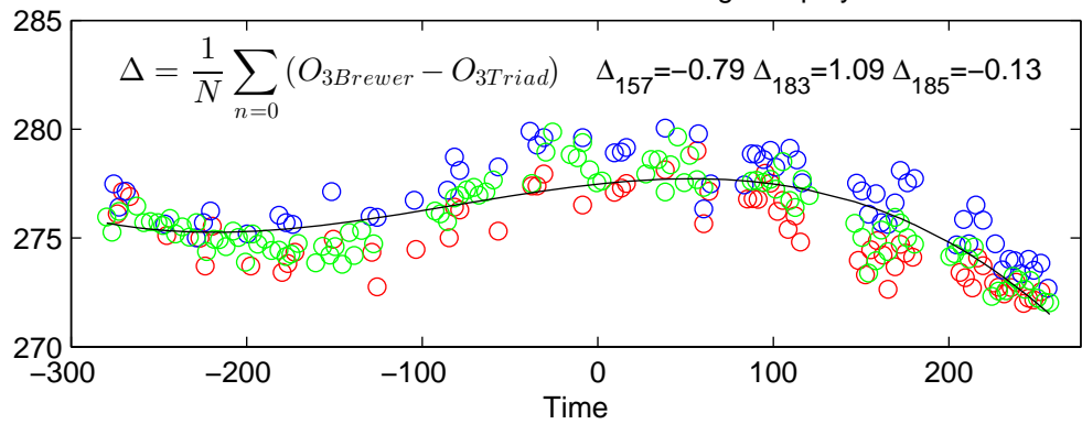
R. Stübi: All measurements fitted 3rd grade polynomial
