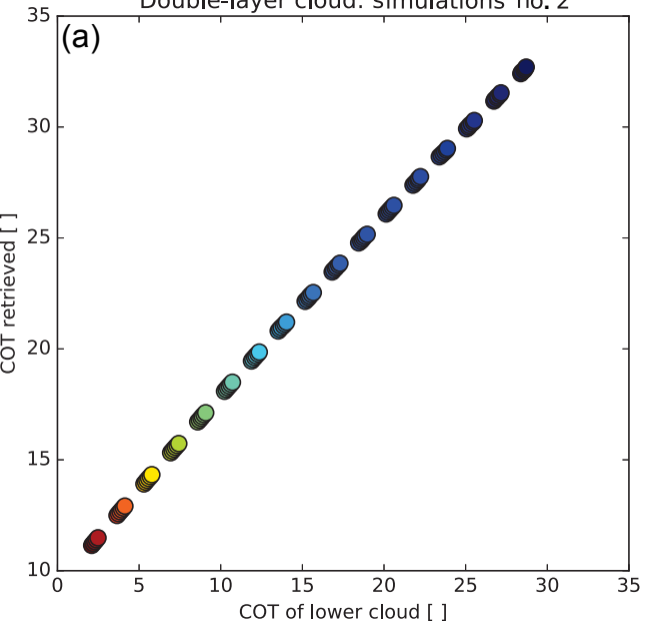
Double-layer cloud: simulations no. 2
