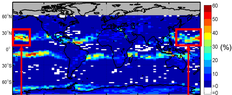
(b) AOD ratio (filter/no filter)
