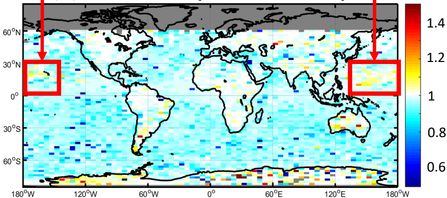
(b) AOD ratio (filter/no filter)
