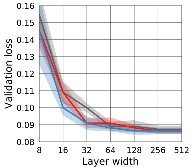
(b) tanh
