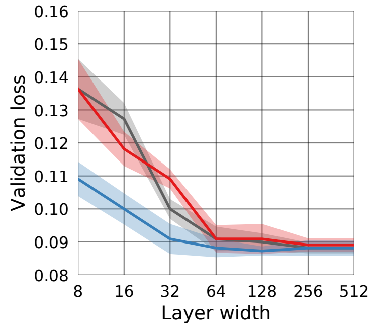
(c) sigmoid
