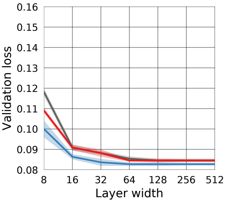
(a) ReLU
