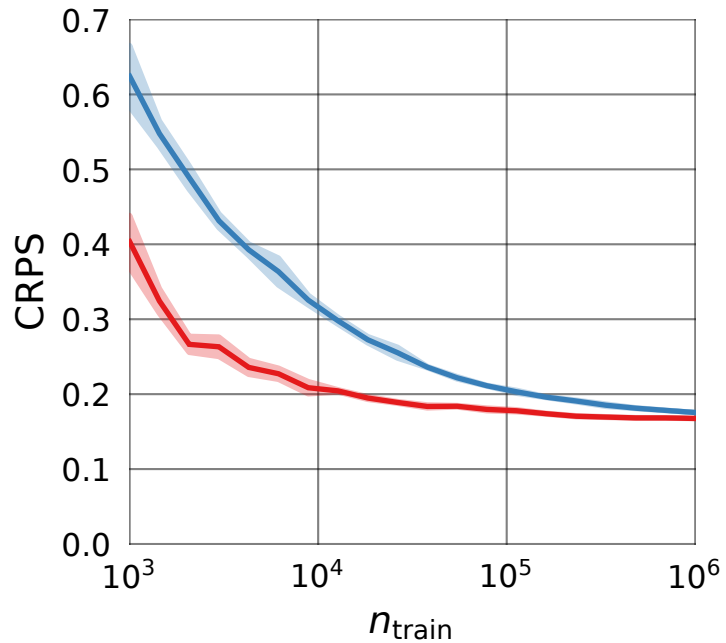
(b) CRPS
