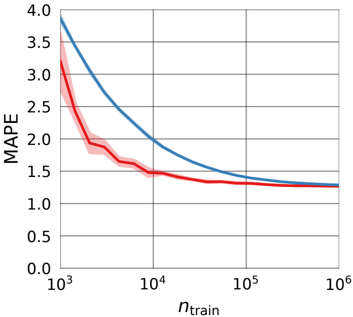
(a) MAPE
