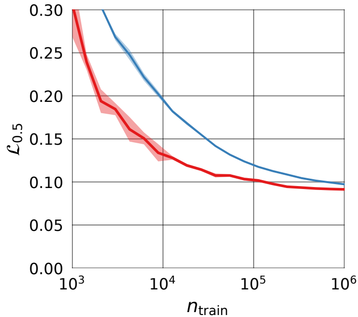
(b) \tau = 0.5
