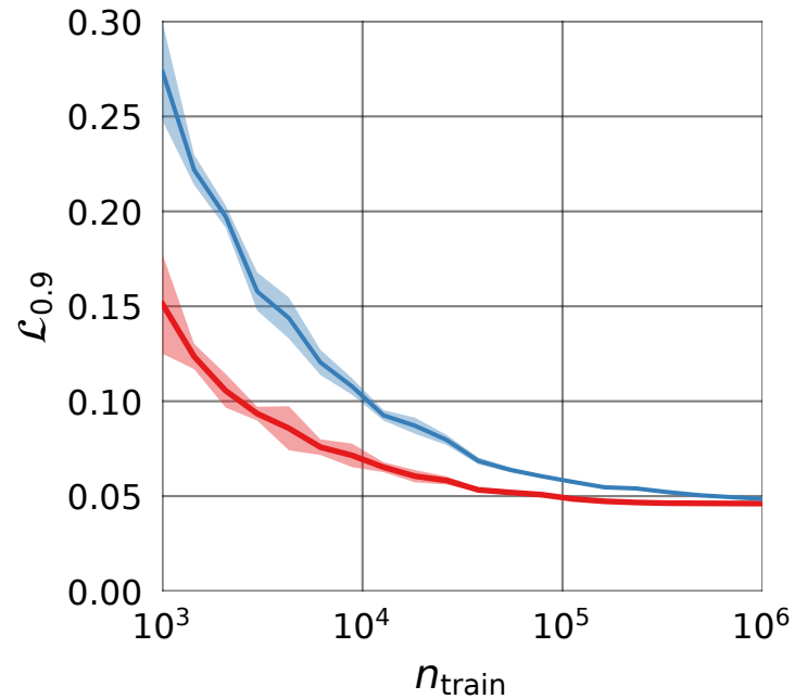
(c) \tau = 0.9
