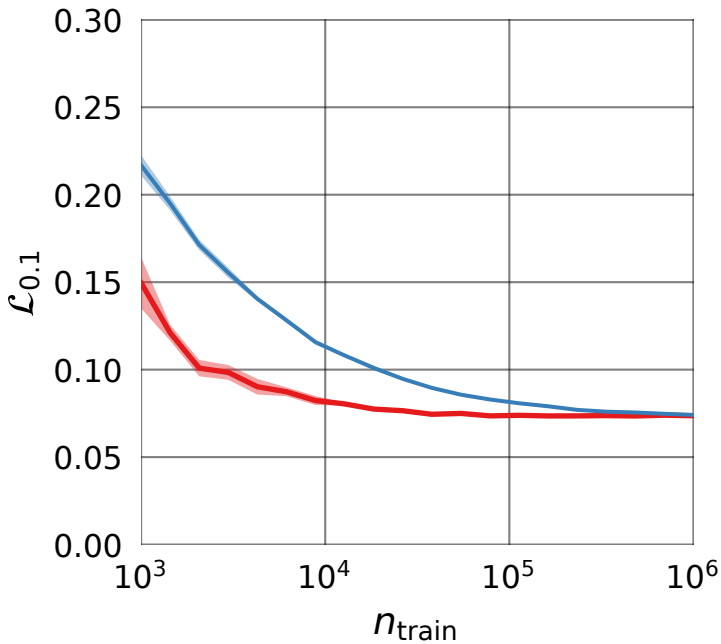
(a) \tau = 0.1
