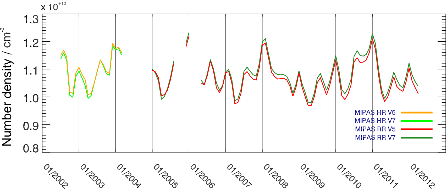
Time series of ozone in 0–10° S at 37 km
