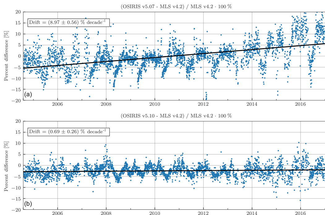
Figure 6. Daily averaged percent difference in zonal mean ozone from 10° S to 10° N at 40.5 km relative to MLS v4.2 for OSIRIS v5.07 (a) and OSIRIS v5.10 (b). The MLS v4.2 data are converted to number density on an altitude grid using ERA-Interim reanalysis pressure and temperature fields. Simple best-fit straight-line drift estimates are shown in black, with uncertainties reported as the 2\sigma values.
