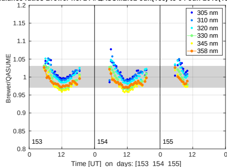
Irradiance ratios Brewer no. 214/QASUME:02-Jun(153) to 04-Jun-2015(155)
