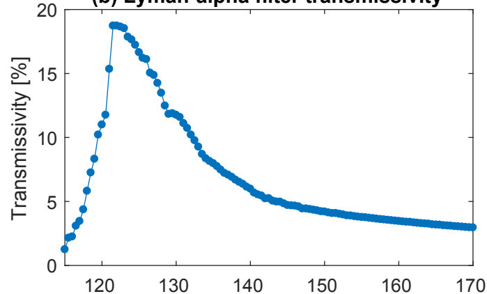
(b) Lyman-alpha filter transmissivity
