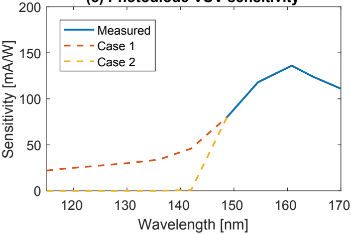
(c) Photodiode VUV sensitivity
