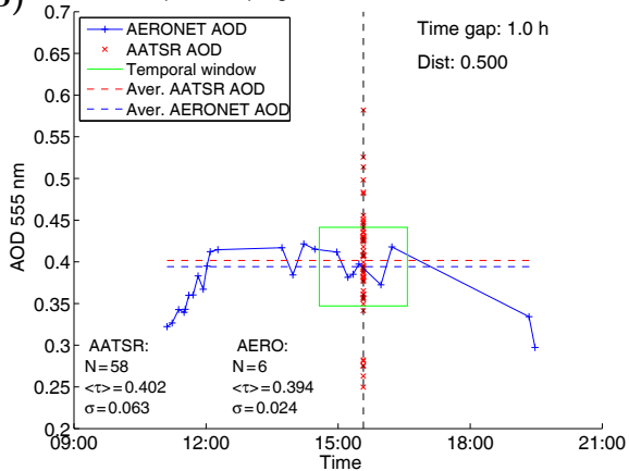
(b) Temporal sampling, DRAGON-ANNEA, 20110722
