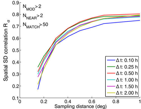
Comparison of spatial standard deviations
