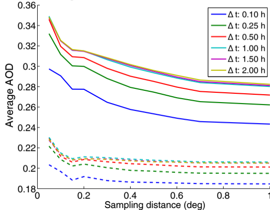
Average collocated AERONET and MODIS AOD
