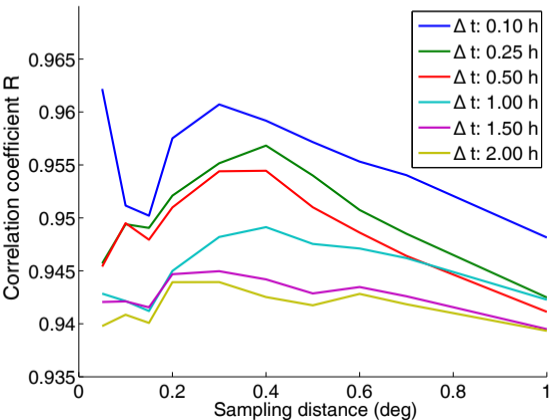
AERONET vs. MODIS AOD comparison
