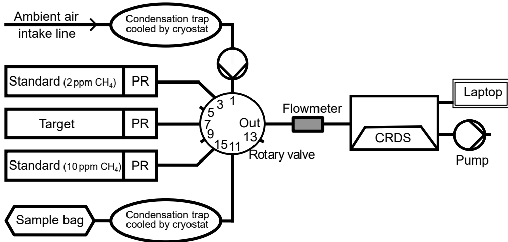
(a) Laboratory set-up
