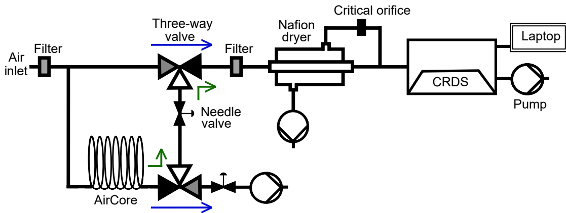
(b) Mobile set-up
