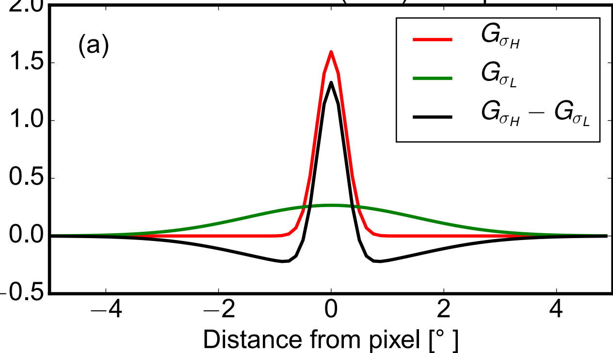
Difference of Gaussians (DoG) band-pass filter
