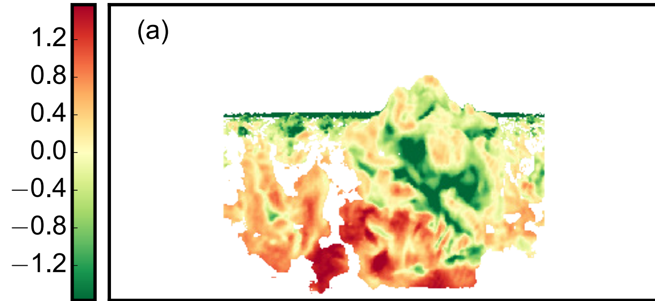
Radiance 2100 nm deviation \Delta L_{2.1} from fit
