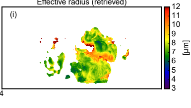
Effective radius (retrieved)
