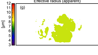
Effective radius (apparent)
