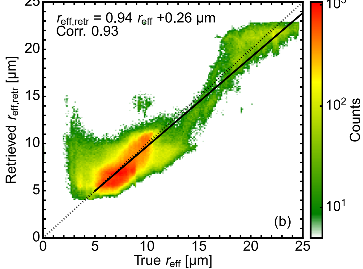
Correlation r_{\text{eff}} vs. r_{\text{eff},\text{retr}} (not included)
