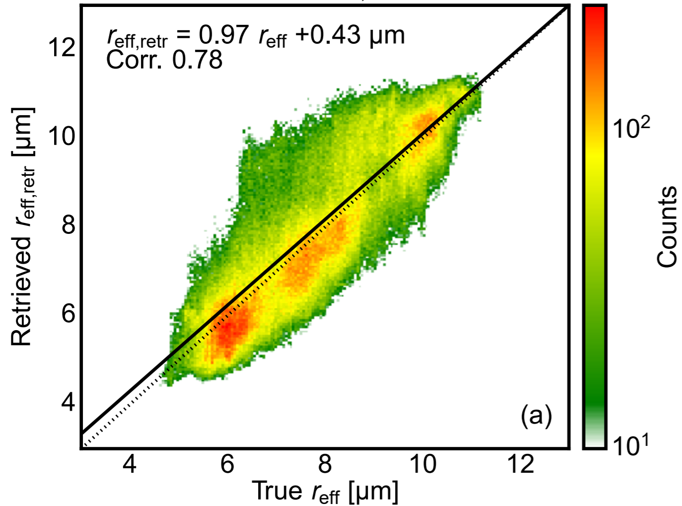
Correlation r_{\text{eff}} vs. r_{\text{eff},\text{retr}} (CCN1000)
