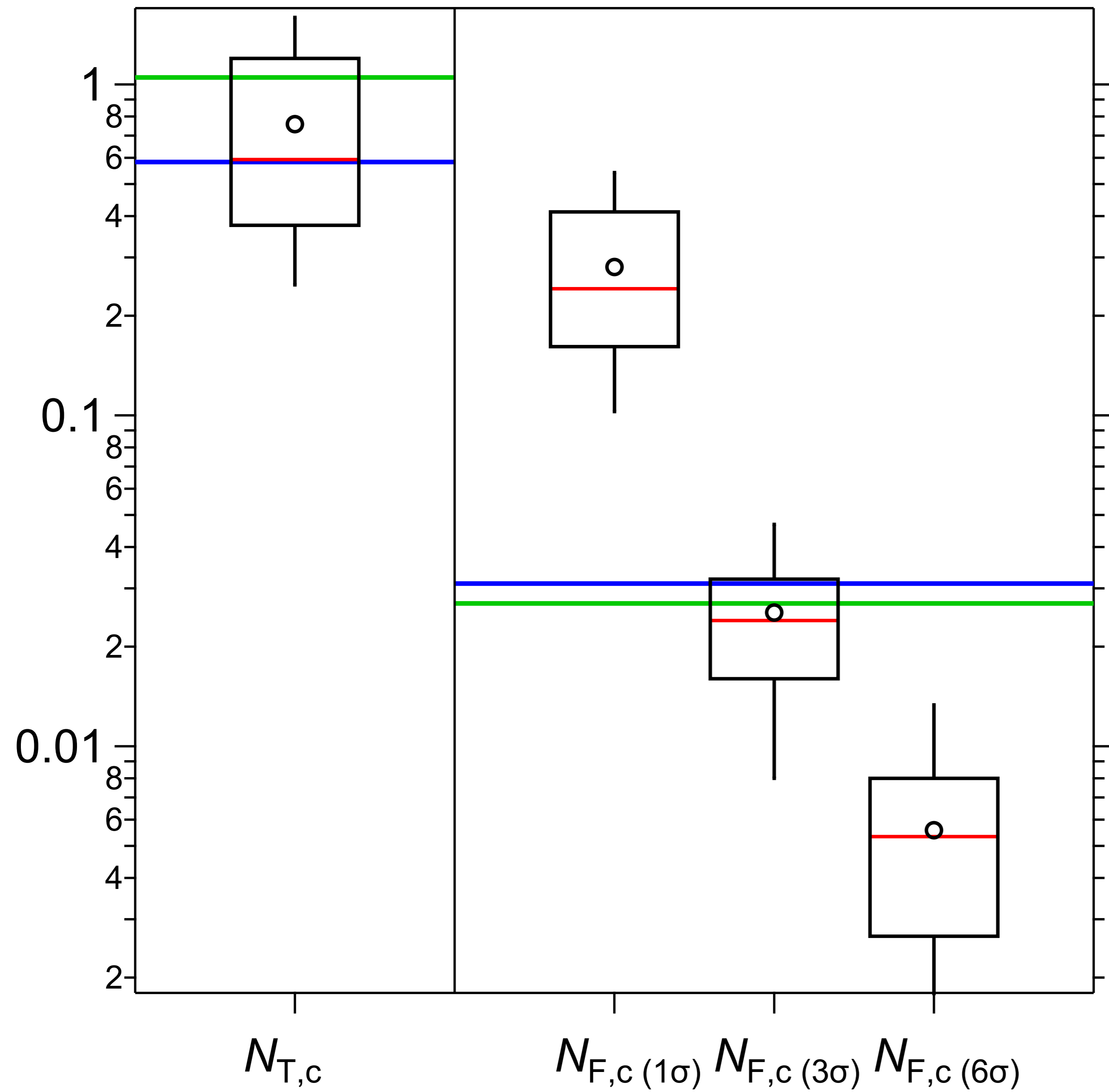
(a) Number concentrations
