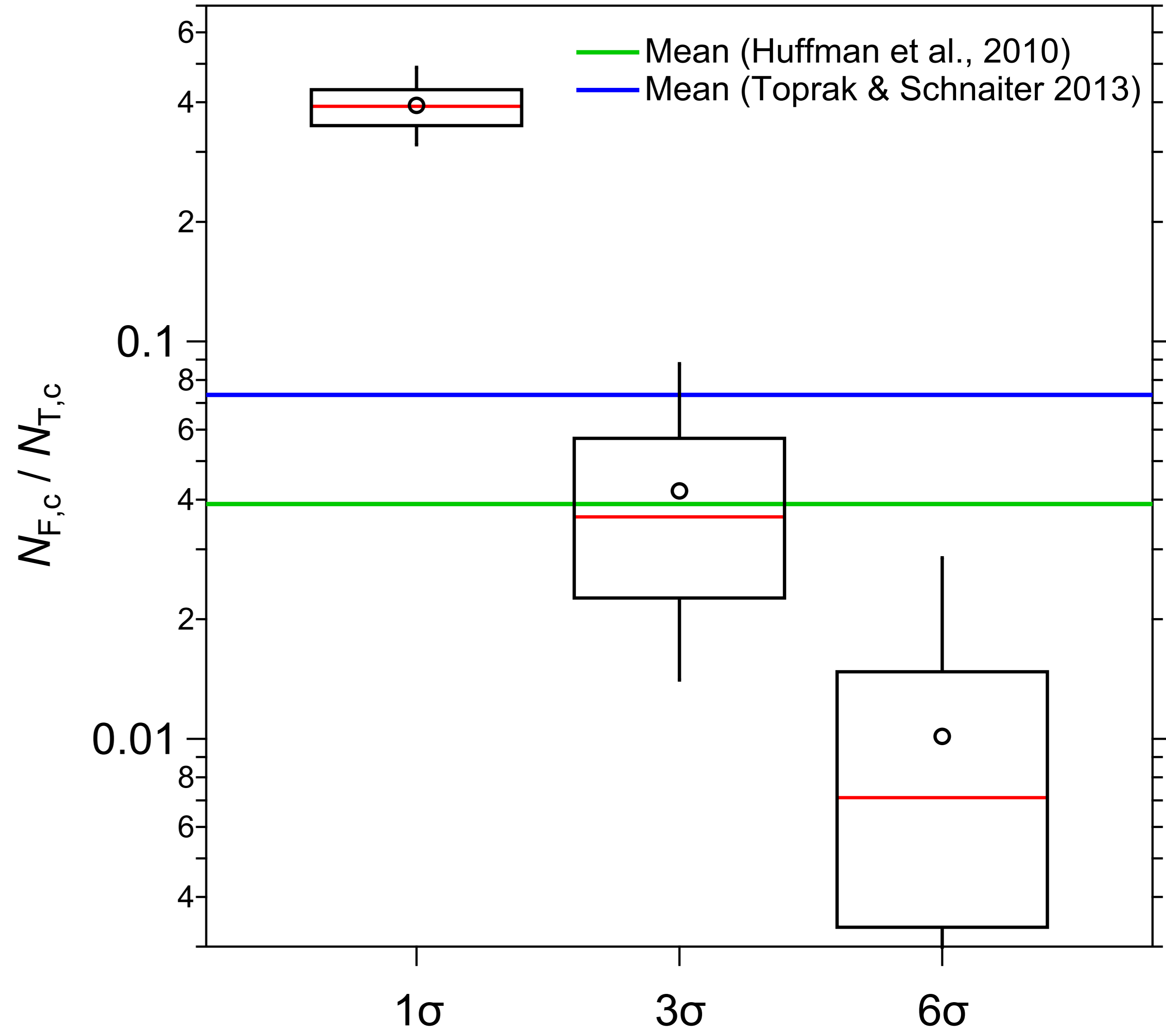
(b) Fluorescent fractions
