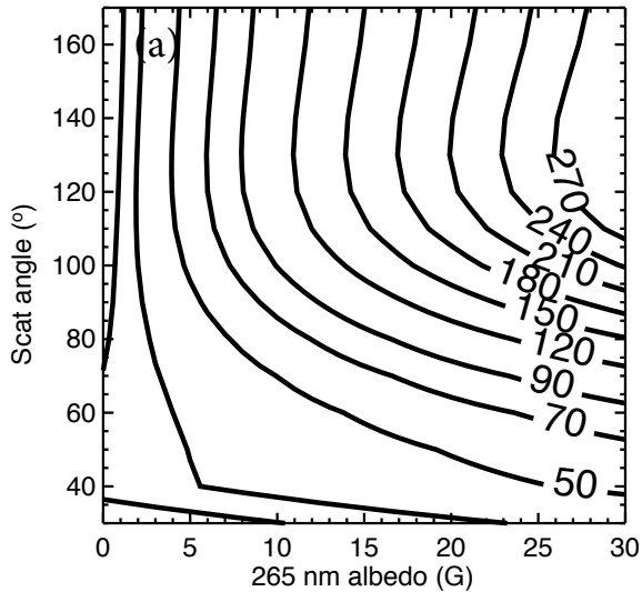
PMC IWC from AIR: Model
