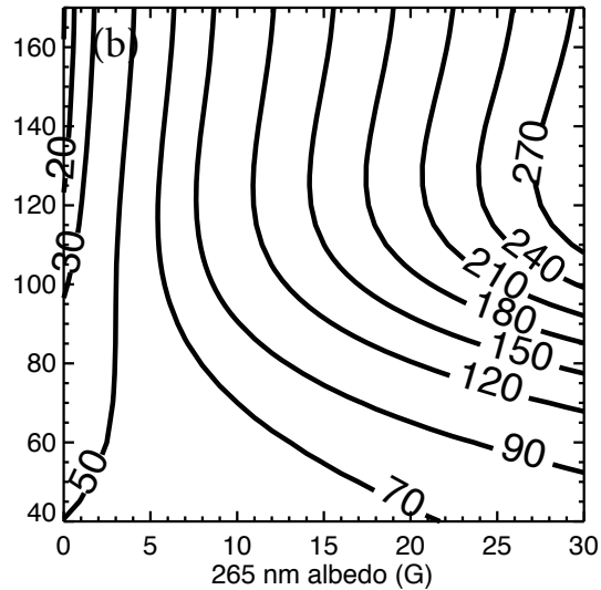
PMC IWC from AIR: SOFIE
