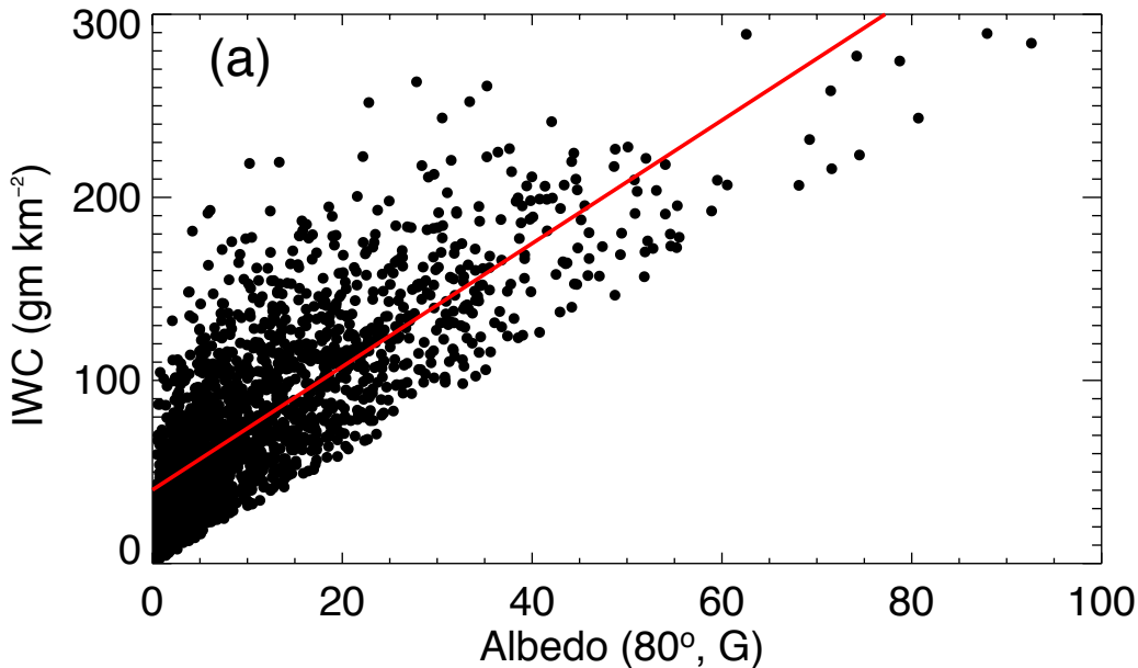
AIM SOFIE IWC vs. 265 nm albedo, sc angle = 80°
