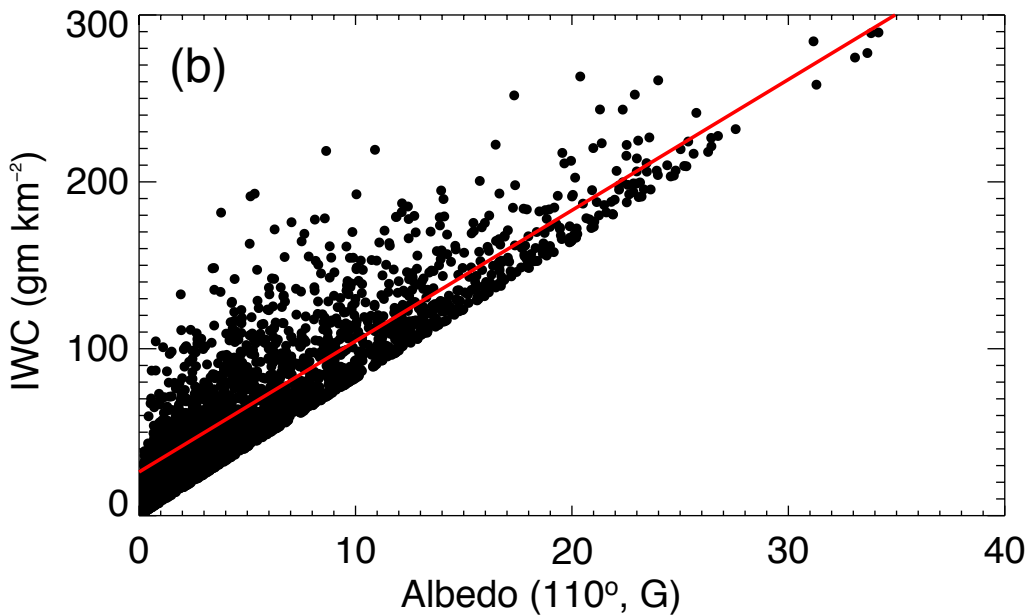
AIM SOFIE IWC vs. 265 nm albedo, sc angle = 110°
