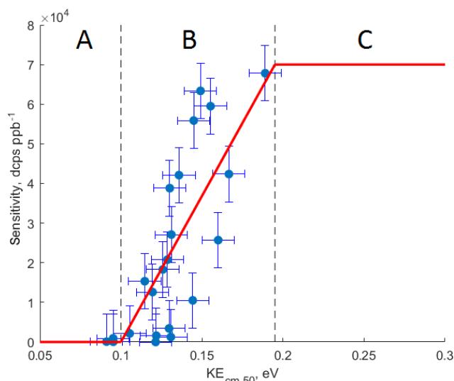
Figure 4. The relationship between calculated kinetic energy of the ammonium–organic clusters KE_{cm50} and measured sensitivity for calibrated compounds. Molecules characterized by KE_{cm50} smaller than 0.10 eV (region A) cannot be detected by NH_4^+ CIMS; for molecules characterized by KE_{cm50} between 0.10 and 0.19 eV (region B) a linear relationship between KE_{cm50} and measured sensitivity is observed; molecules characterized by KE_{cm50} greater than 0.19 eV (region C) are detected at the “kinetic sensitivity”.
