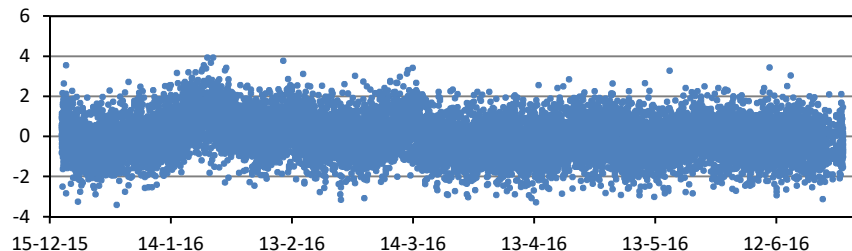
CO target (CA07080): 30 s means (ppb) minus their mean
