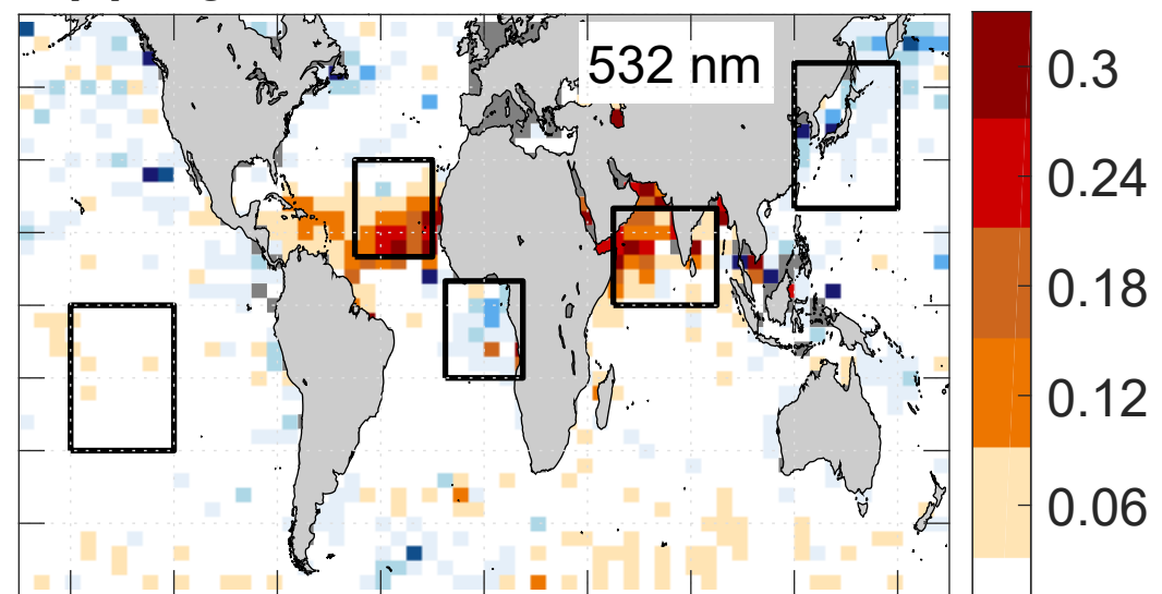
(b) Nighttime CALIOP V4 - SODA
