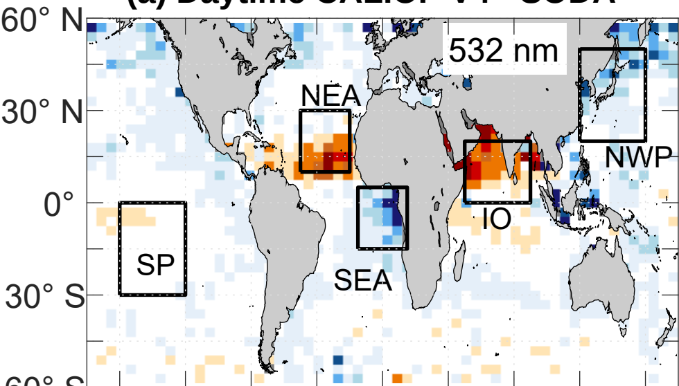
(a) Daytime CALIOP V4 - SODA
