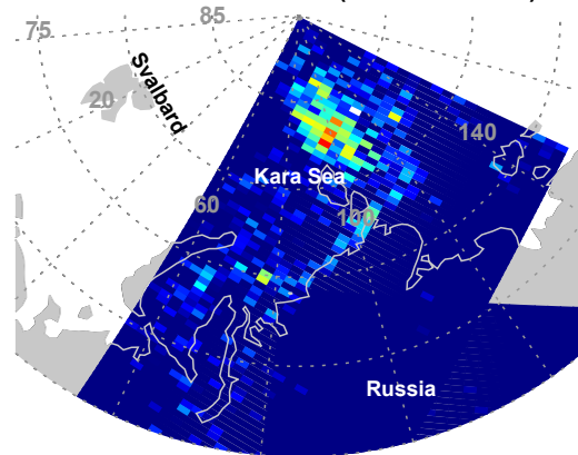
(c) GOME-2B BrO VCD (orbit no. 28847)
