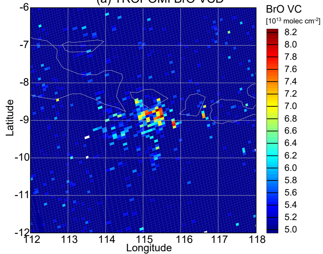
(a) TROPOMI BrO VCD
