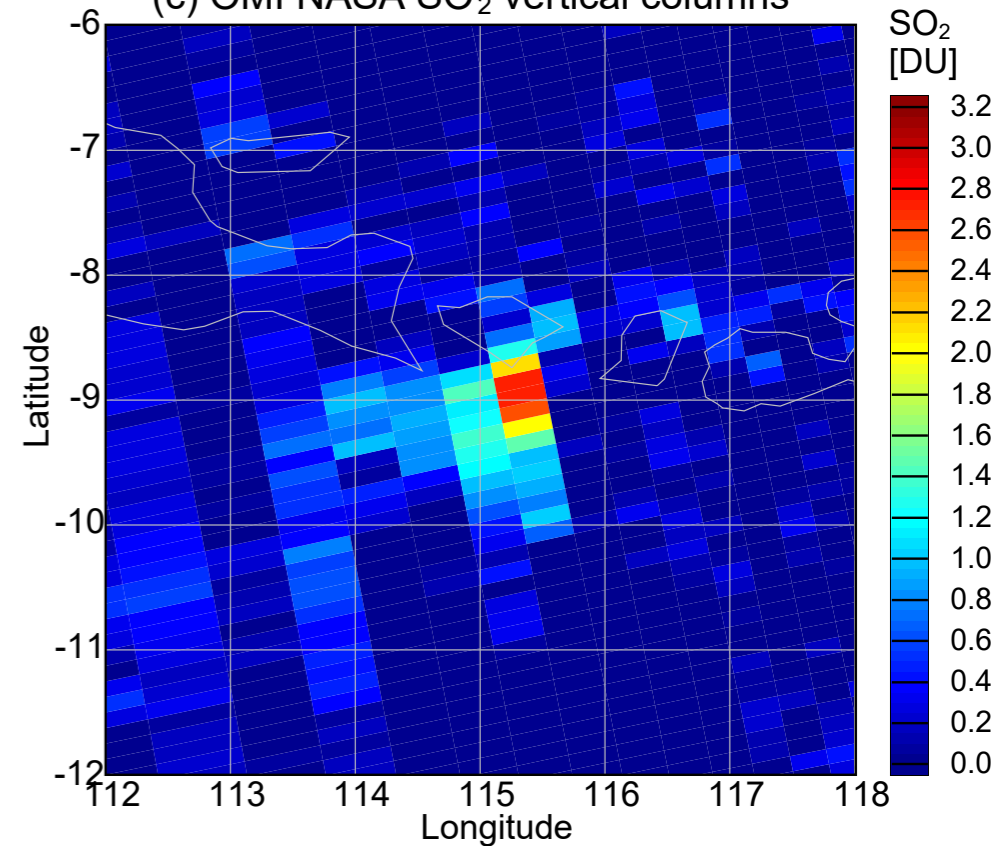
(c) OMI NASA SO 2 vertical columns
