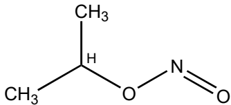
Isopropyl nitrite
