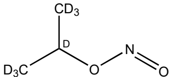
Isopropyl nitrite-d 7
