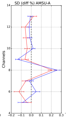
(c) AMSU-A
