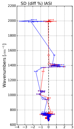
(a) IASI
