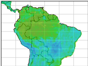
(a) Baseline, 2007-09-23
