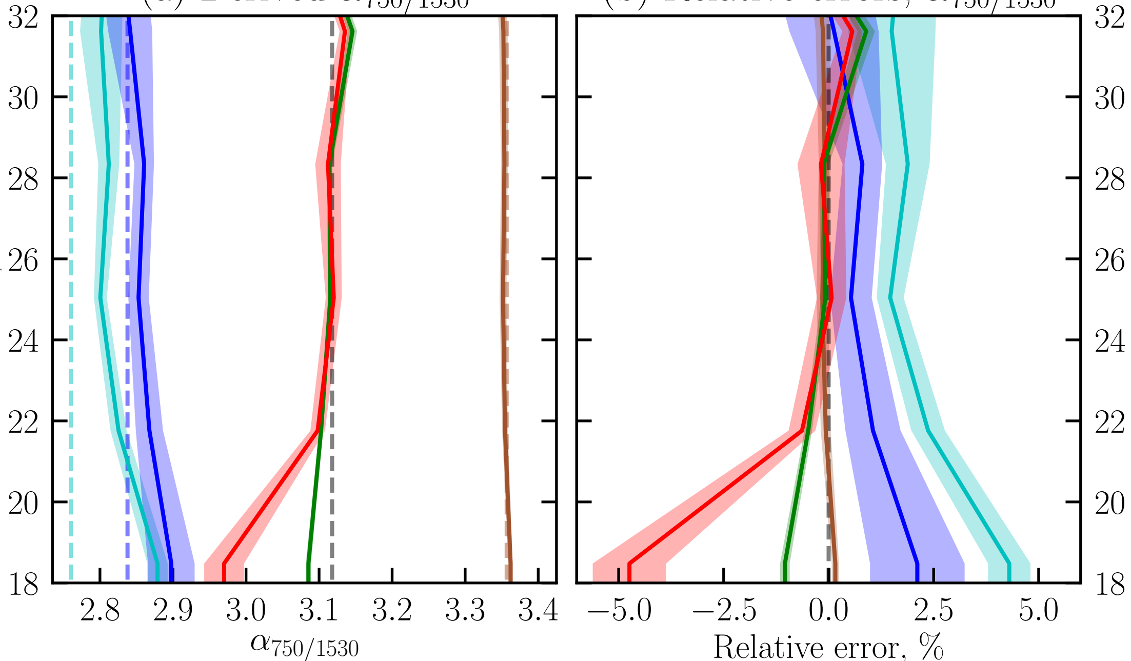
(a) Derived \alpha_{750/1530}
