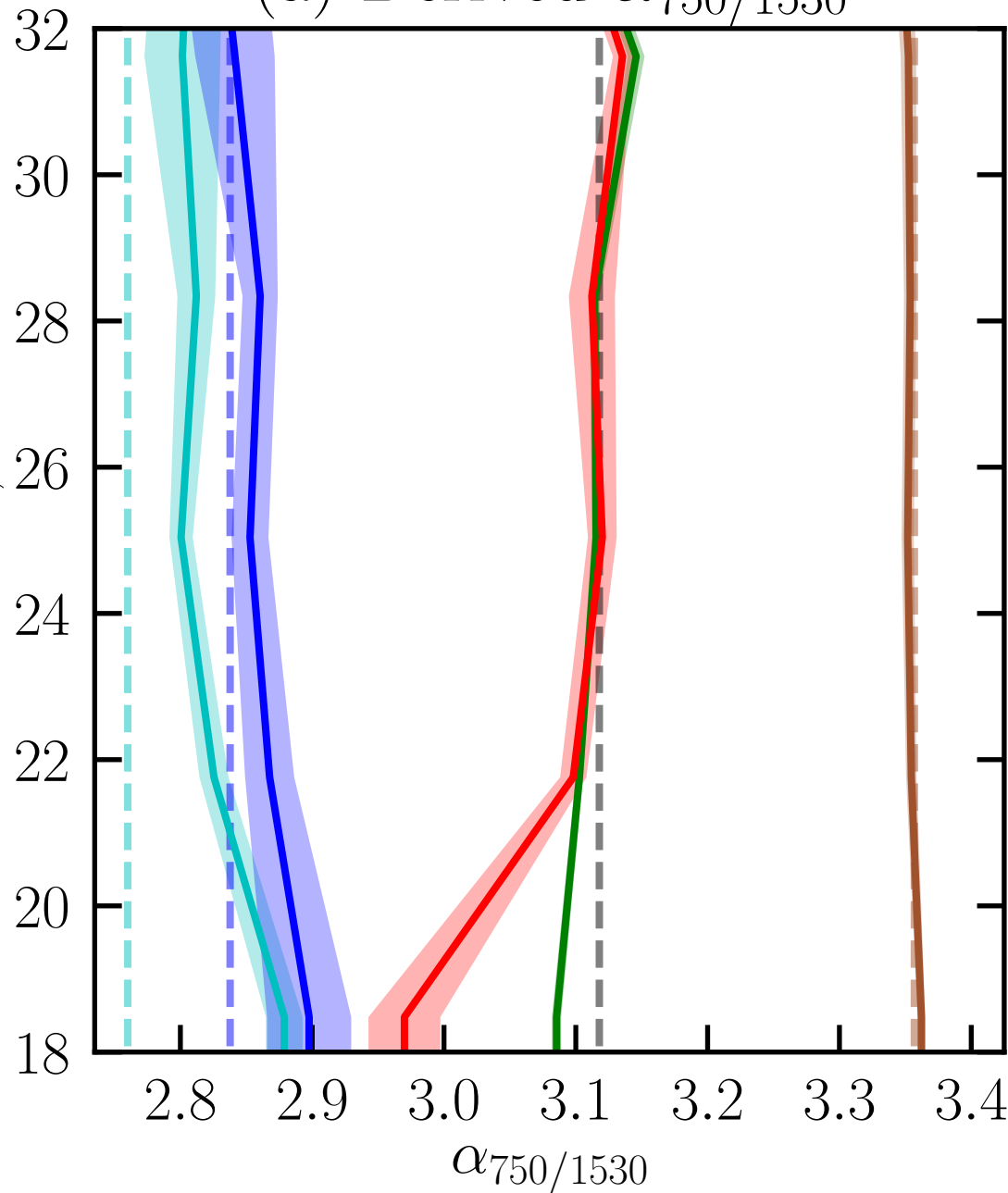
(a) Derived \alpha_{750/1530}
