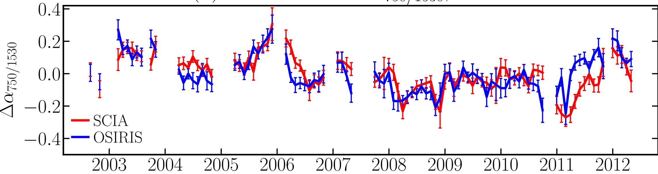
(b) Deseasonalized \alpha_{750/1530} , 21.3 km
