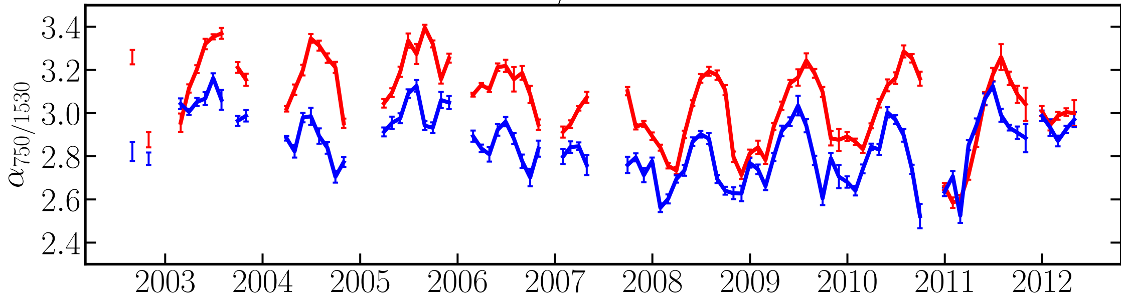
(b) Deseasonalized \alpha_{750/1530} , 21.3 km
